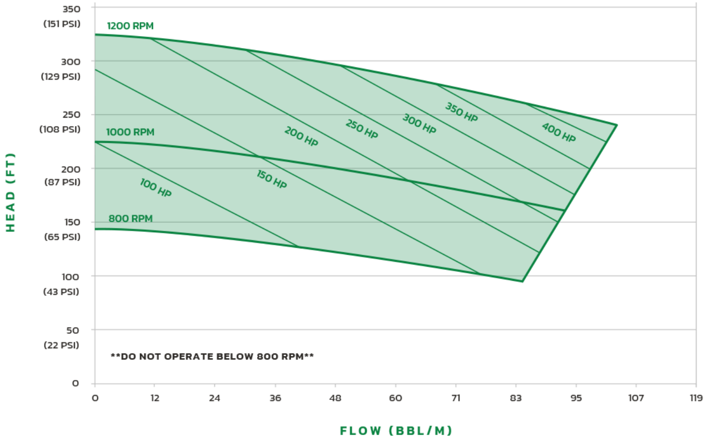
12X10X25 - WATER PERFORMANCE - ENCLOSED IMPELLER
