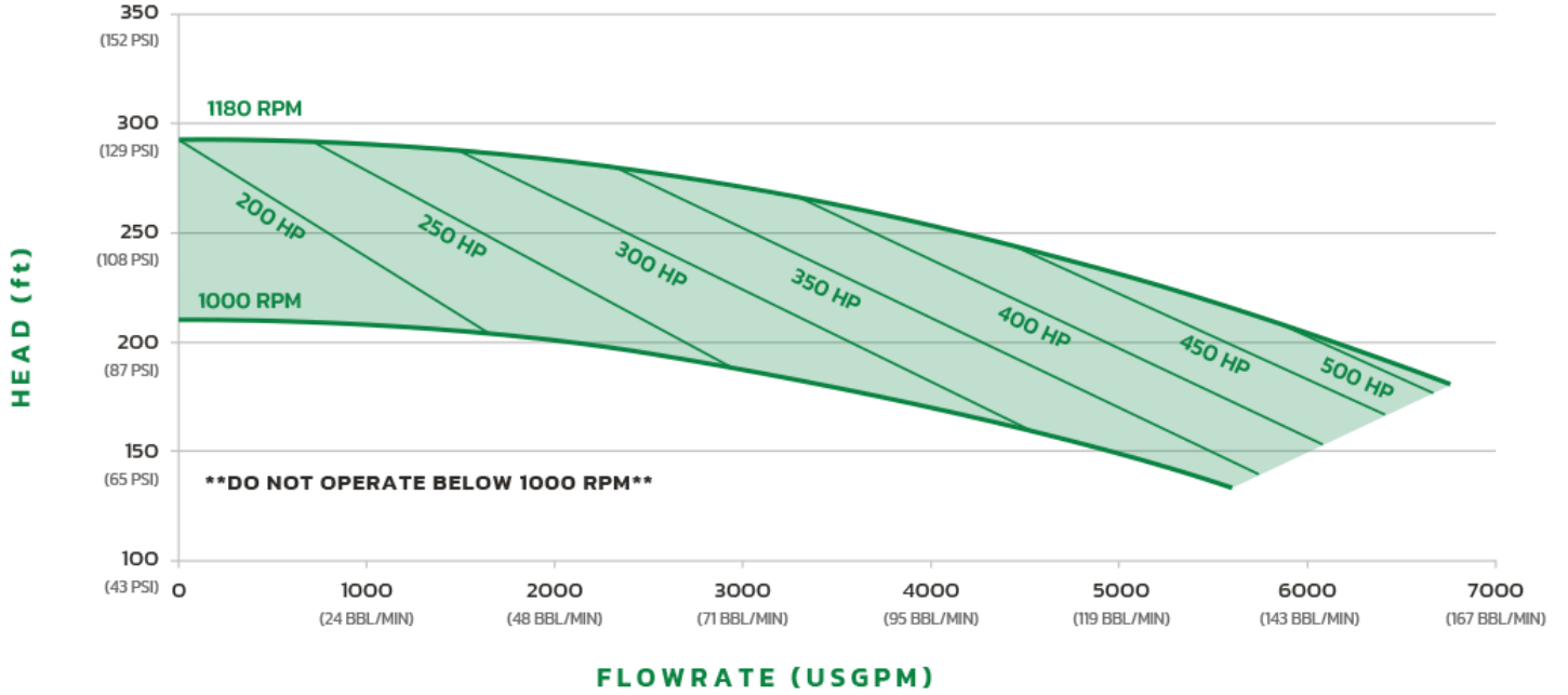
WATER PERFORMANCE - ENCLOSED IMPELLER - STANDARD VOLUTE
